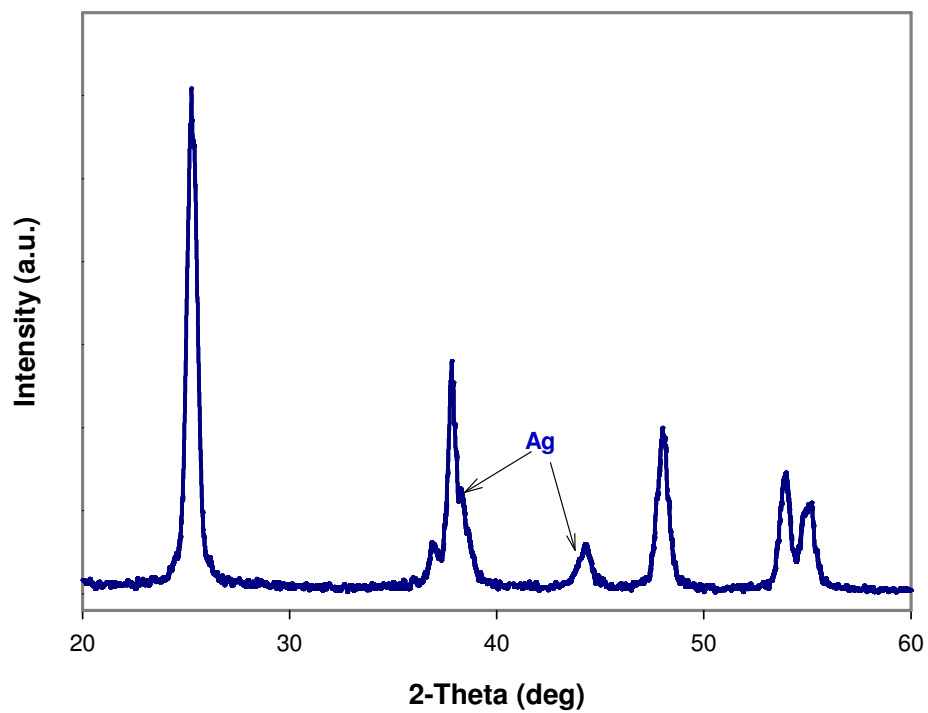
Figure S10. XRD pattern hybrid Ag-TiO 2 NCs with Ag clusters of size between 5 to 10 nm (corresponding TEM image in Figure 3A).
