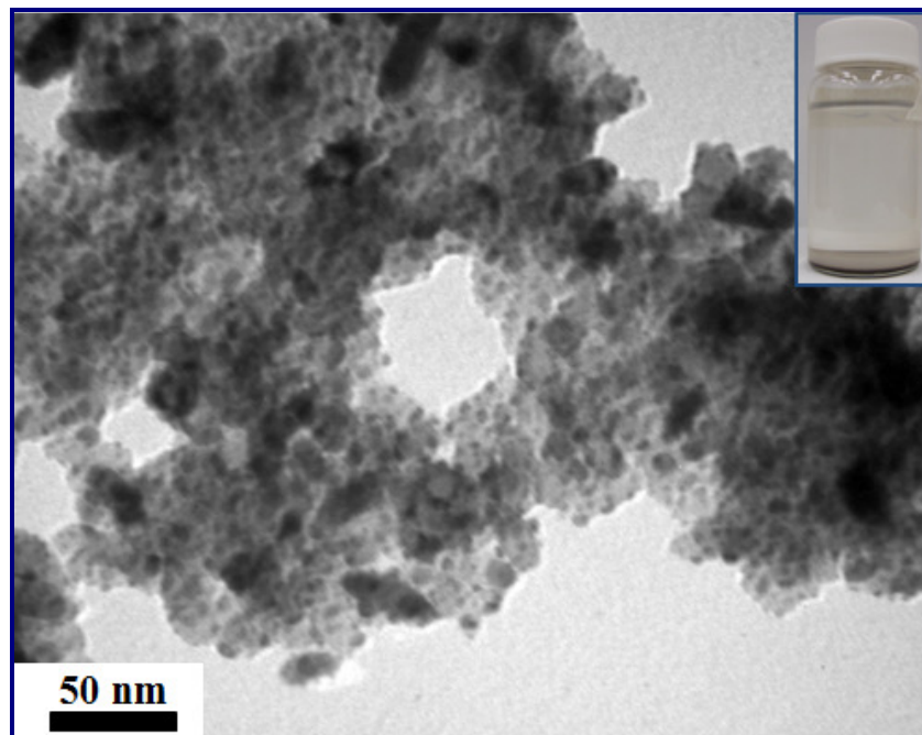
Figure S5. TEM image of hybrid Ag-TiO 2 NCs synthesized without additional OA and irradiated for 60 minutes. Insert is the photo of the mixture after reaction. The hybrid Ag-TiO 2 NCs are precipitated and leave behind a blank solution indicating that the Ag clusters existed only on TiO 2 NC surface.
