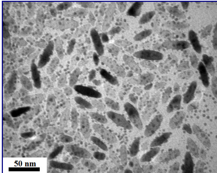
Figure S7. TEM image of hybrid Ag-TiO 2 NCs formed by adding a small amount of oleylamine to the hybrid Ag-TiO 2 NC solution, which is obtained by irradiating a solution of TiO 2 nanorods containing silver nitrate salt for 40 minutes, and irradiating for 60 minutes.
