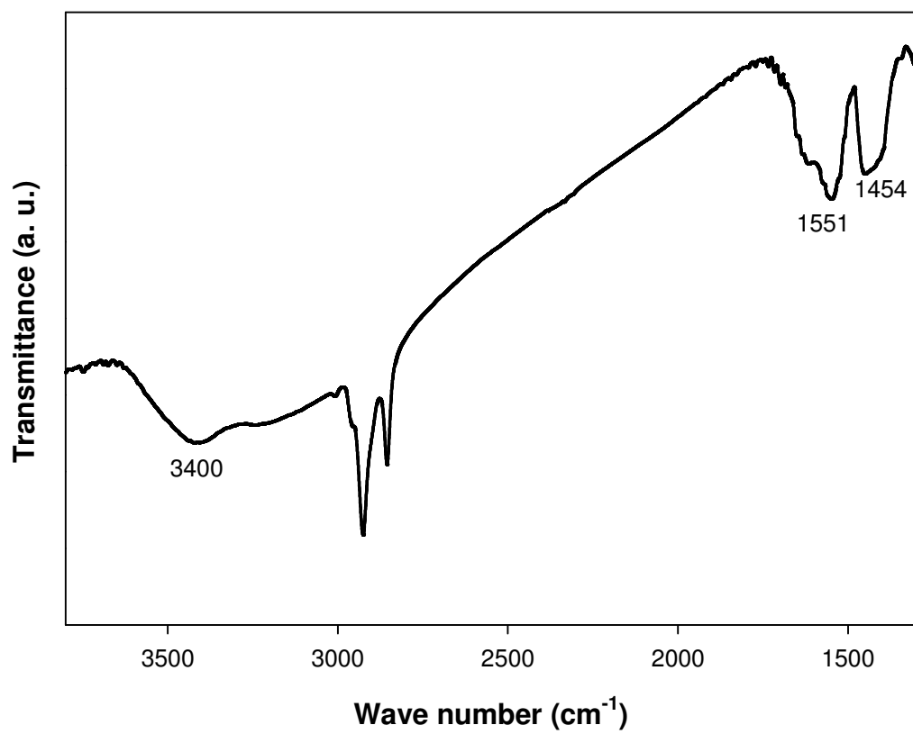
Figure S9. FTIR spectrum of as-made TiO 2 NCs used as support for the deposition of Ag clusters
