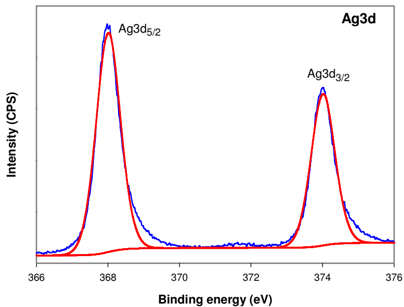
Figure S2. Ag 3d X-ray photoelectron spectrum of the hybrid Ag-TiO 2 NCs (2.6 % mol. Ag) synthesized by irradiating of TiO 2 nanorods solution containing silver nitrate salt for one minute with no additional OA.
