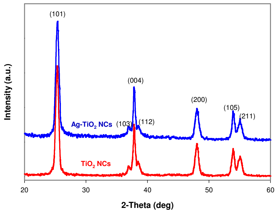
Figure S3. XRD patterns of the TiO 2 nanorods and hybrid Ag-TiO 2 NCs (2.6 % mol. Ag) synthesized by irradiating a solution of TiO 2 nanorods containing silver nitrate salt during one minute without additional OA. The two XRD patterns are similar, indicating a very small size of Ag clusters.
