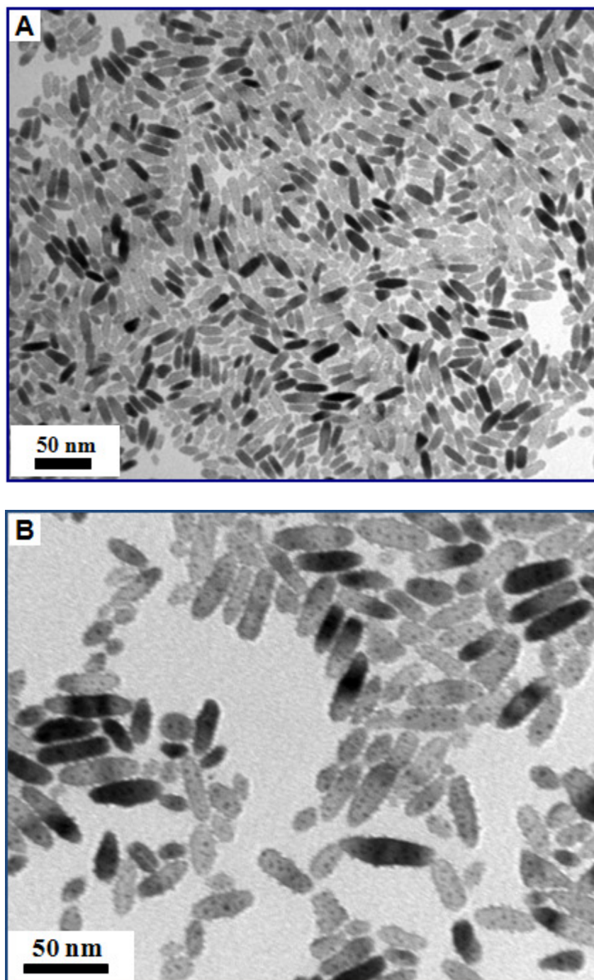
Figure S1. TEM images of the hybrid Ag-TiO 2 NCs (2.6 % mol. Ag) synthesized by irradiating a solution of TiO 2 nanorods containing silver nitrate salt for one minute with no additional OA. (A) low magnification image, and (B) image taken of a low particle concentration region on the grid, however, no separated Ag clusters were observed.
