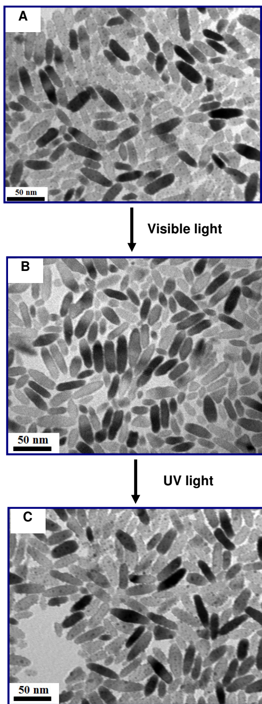
Figure S11. TEM images of the hybrid Ag-TiO 2 NCs synthesized by irradiating a solution of TiO 2 nanorods containing silver nitrate salt for one minute with no additional OA before exposing to visible light (A), after exposing to visible light for one day (B), and after exposing to visible light for one day and re-exposing to UV light for 1 minute (C).
