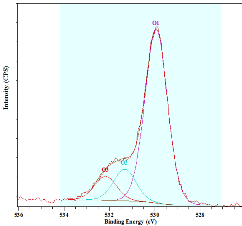
Figure S8. O1s X-ray photoelectron spectrum of the as-synthesized TiO 2 NCs.
