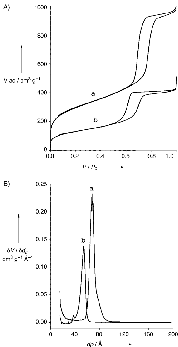
Figure 1. N_2 adsorption/desorption isotherms of nitrogen at -196^\circ\text{C} (A) and Barrett–Joyner–Halenda (BJH) pore diameter distributions calculated from the desorption branch of the isotherm (B) for a) parent MesoAS, b) ZSM-5-coated MesoAS.
